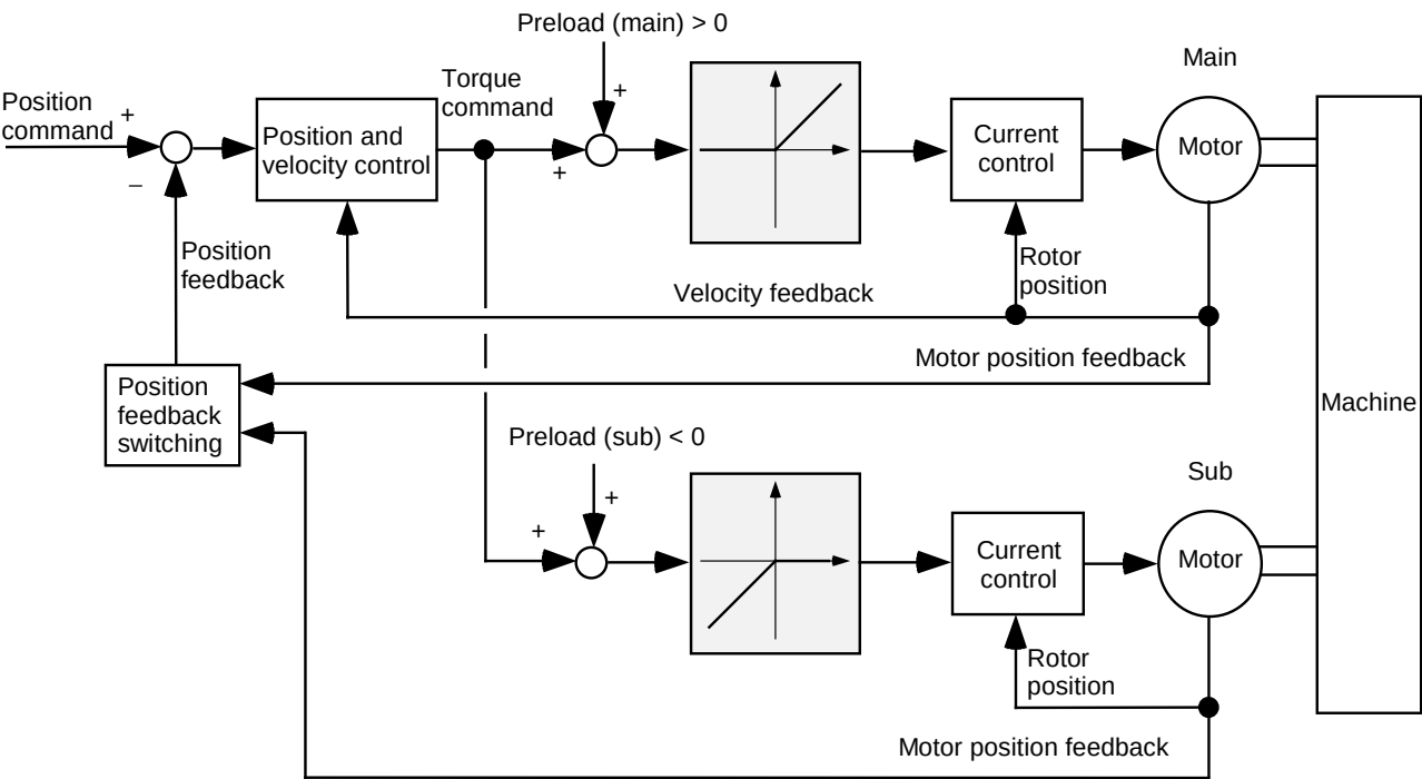
Fig. 4.17.7 (c) Servo block diagram (full preload function)
