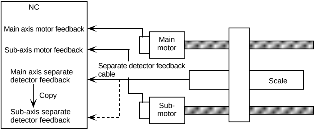
Fig. 4.17.6 Full-closed loop feedback sharing function
