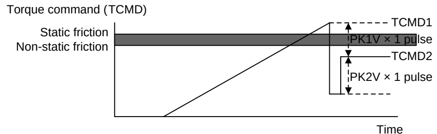
Fig. 4.7 (d) Torque commands (when there is no overshoot)
