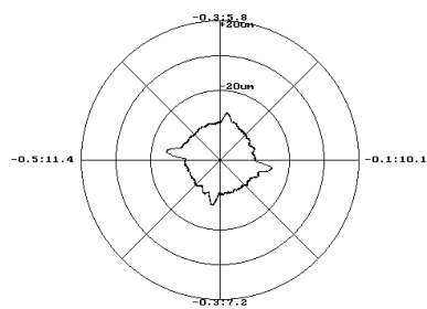
Circle before feed-forward adjustment
