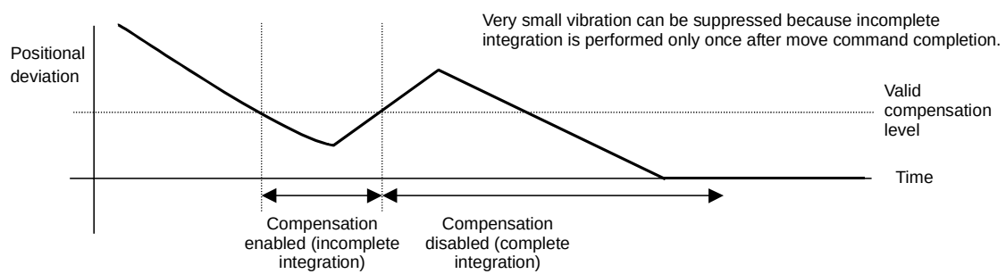
Fig. 4.7 (i) Overshoot compensation type 2
