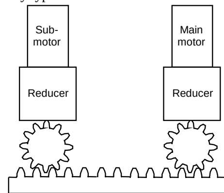
Fig. 4.17.10 (c) Example of tandem control (machine system supporting back-feed)
