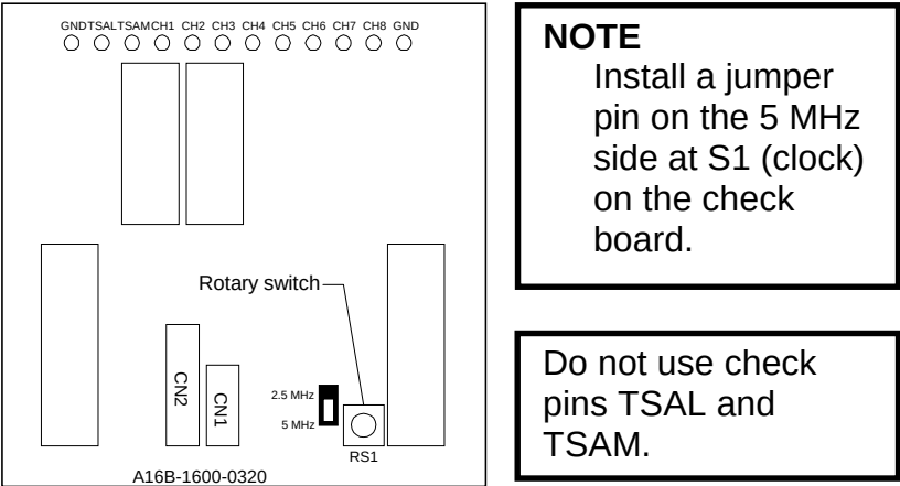
Fig. 4.19 (c) Connector layout on servo check board C (A06B-6057-H602)
