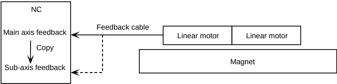
Fig. 4.17.5 Motor feedback sharing function
