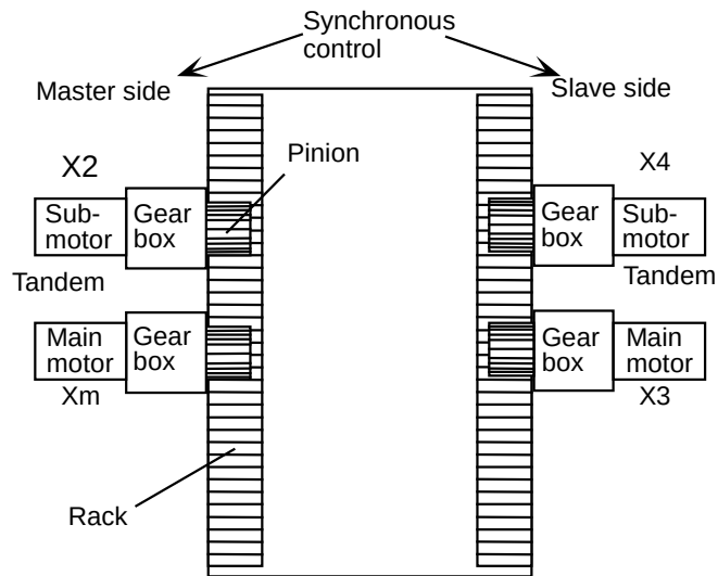
Fig. 4.17.7 (e) Synchronous tandem control
