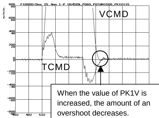
Fig. 3.4.4 (g) After PK1V adjustment
